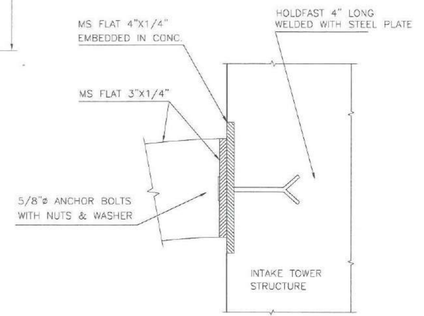
DETAIL - 1
