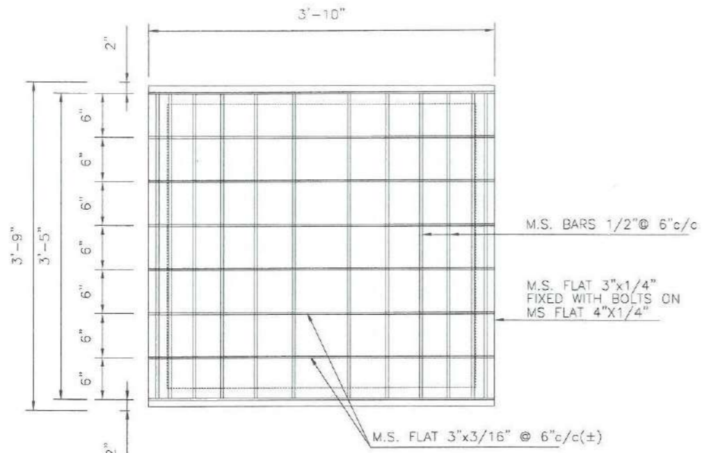
SECTION A-A LOWER TASHRACK ELEVATION
