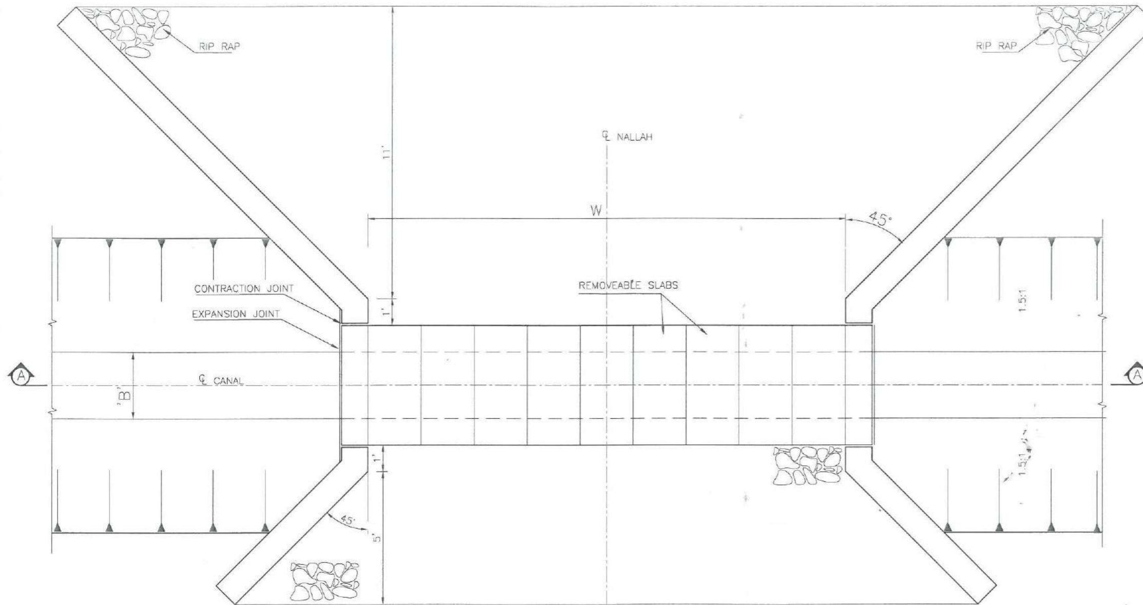
PLAN
