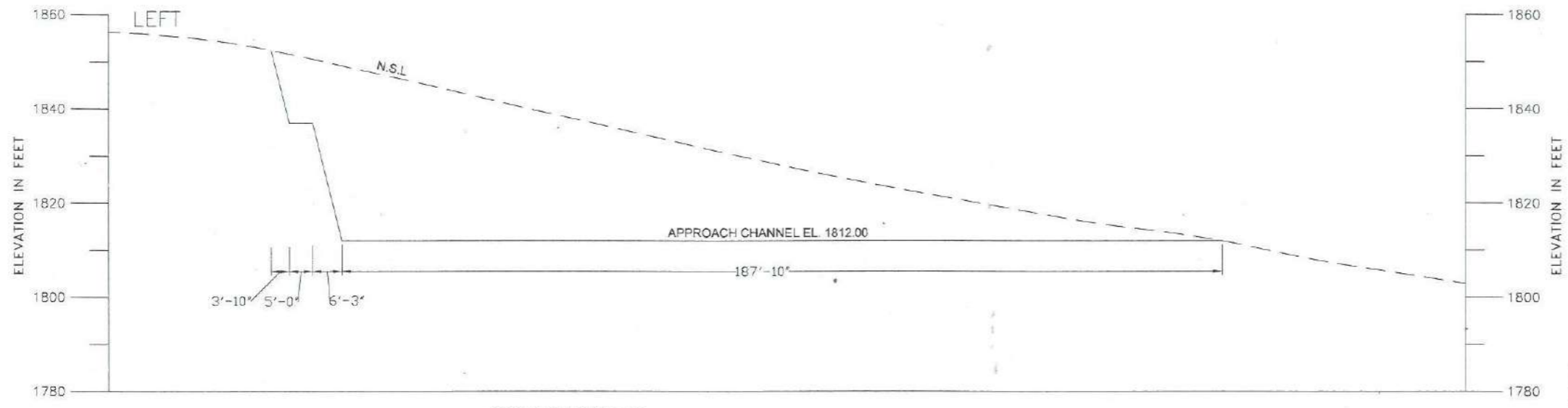
SECTION B-B
