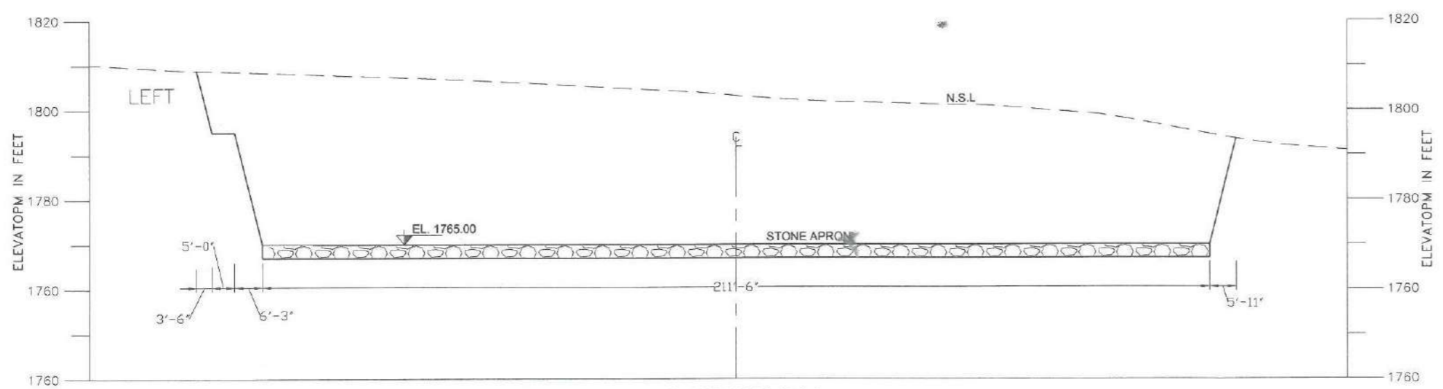
SECTION H-H
