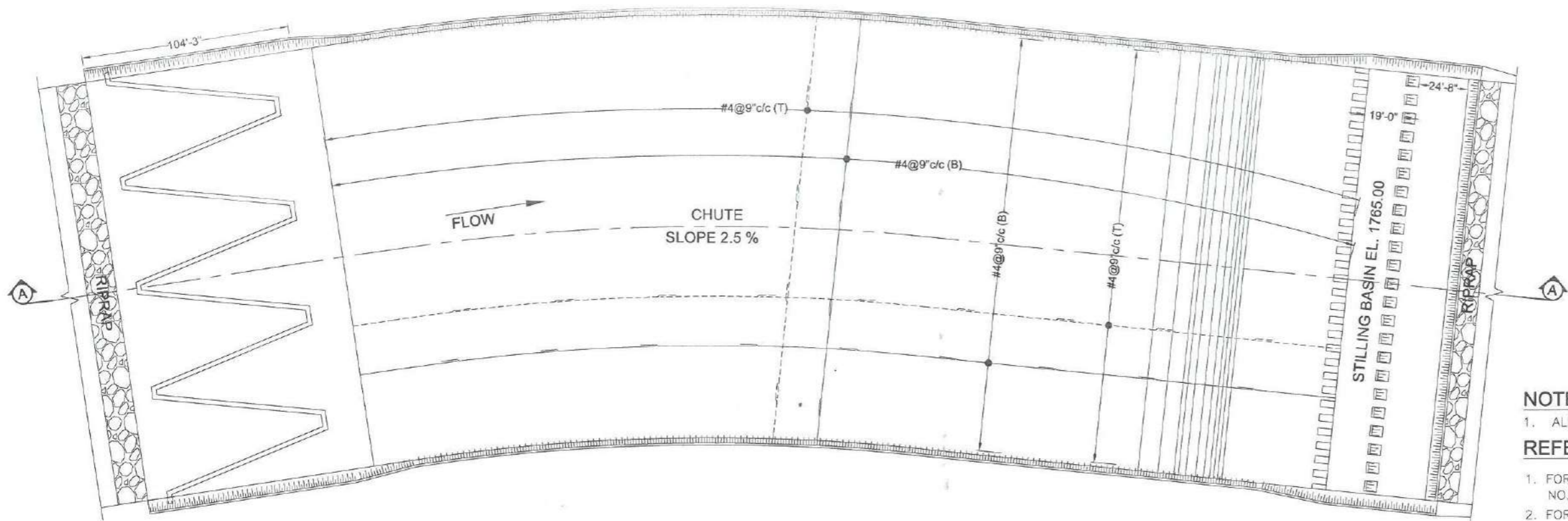
SPILLWAY PLAN
