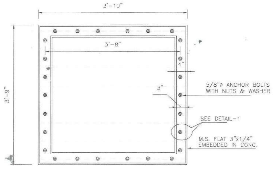
SECTION C-C LOWER TASHRACK FRAME
