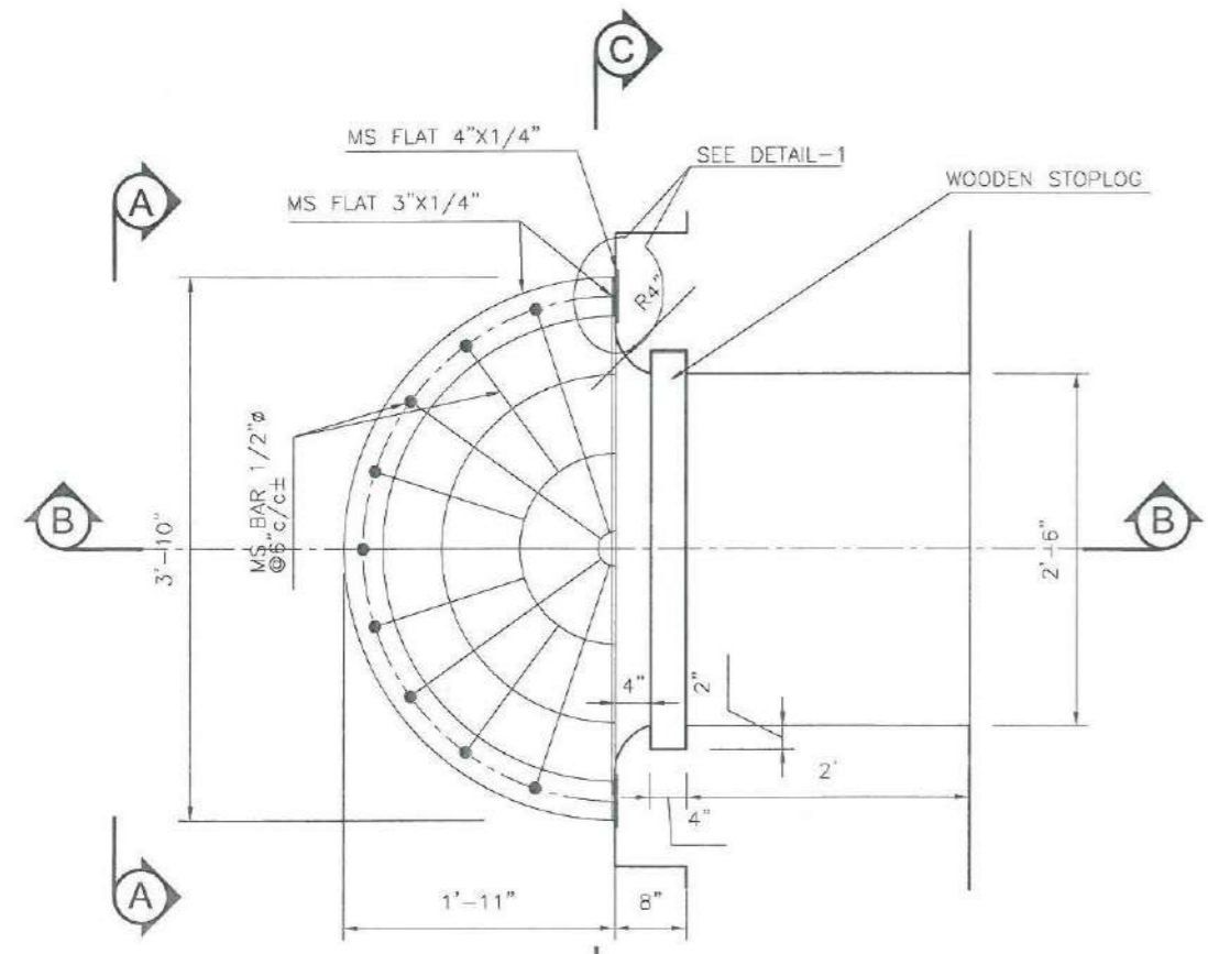
LOWER TASHRACK PLAN
