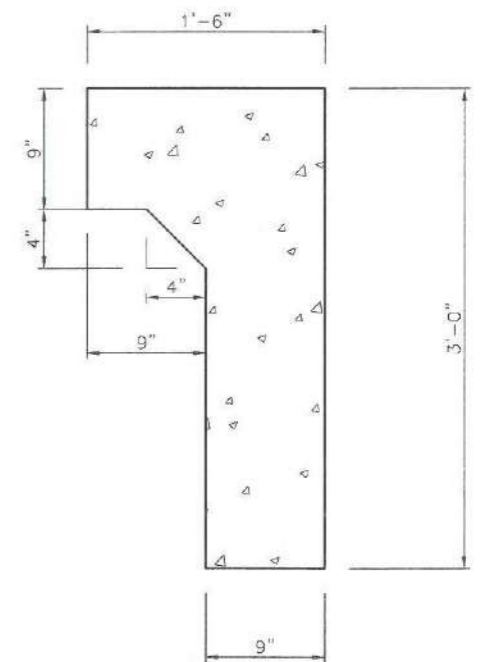
IMPACT WALL DETAIL
