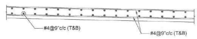
DETAIL (A)
