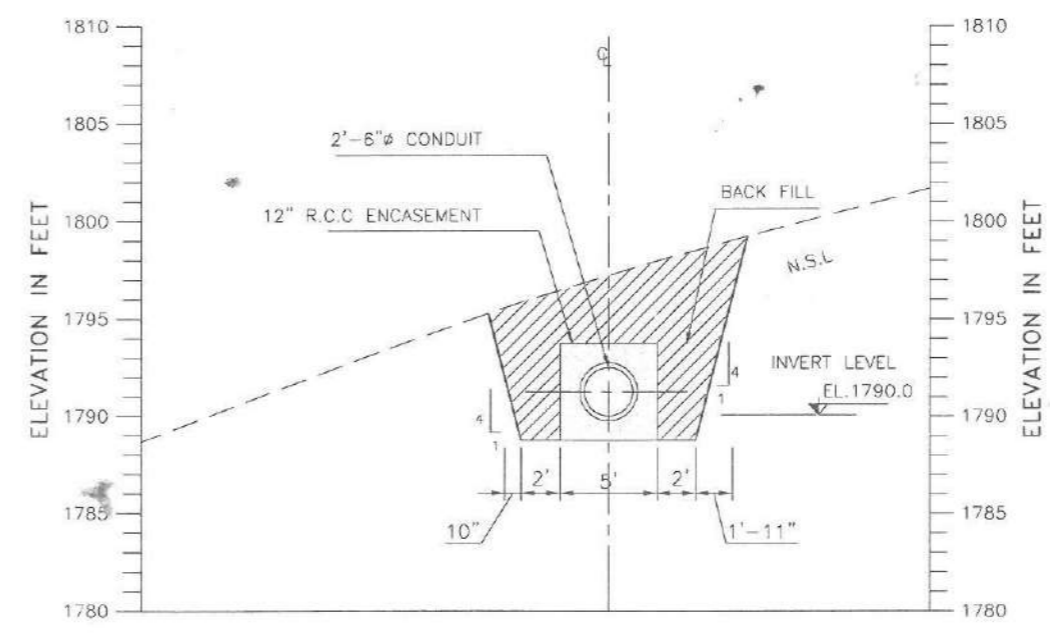
SECTION E-E
