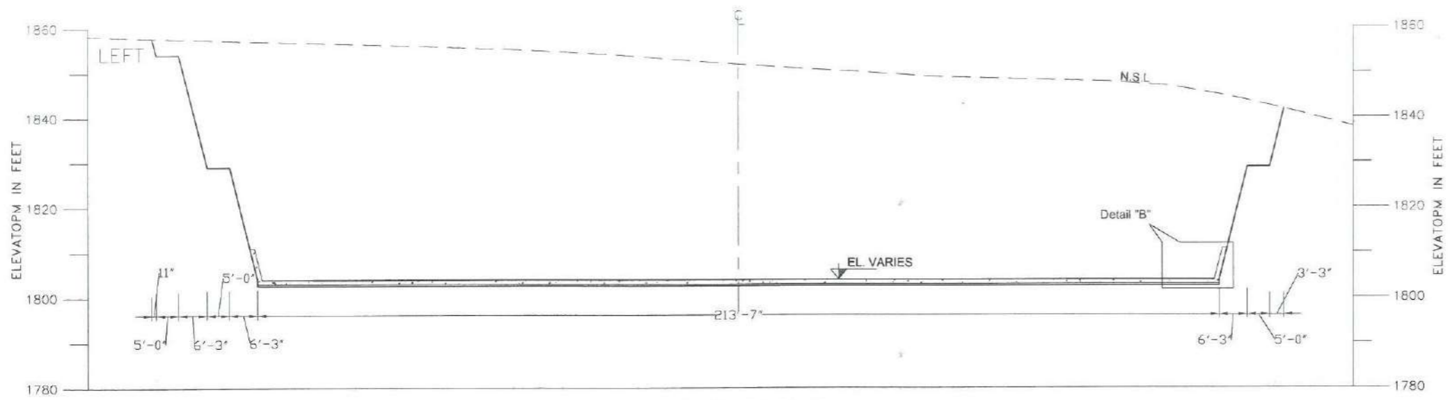
SECTION F-F
