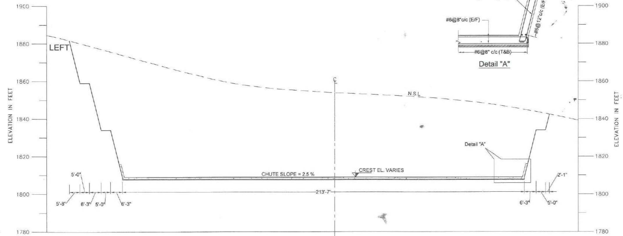
SECTION E-E
