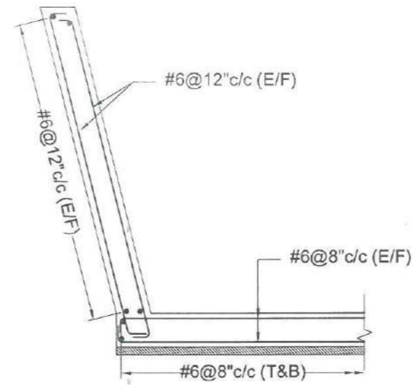
SECTION 3-3
